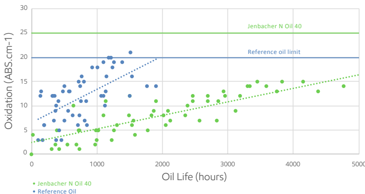
Oxidation Performance - Type 6F Engine
